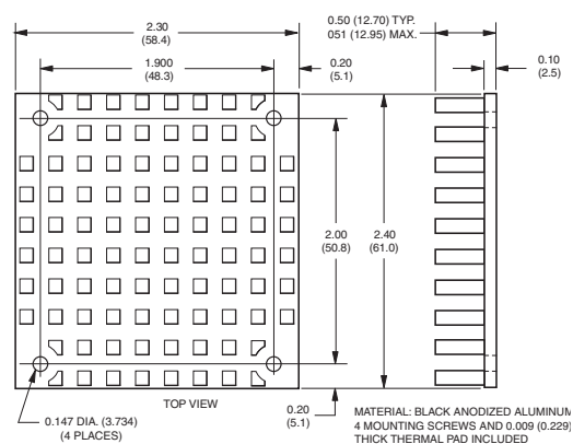
Optional Heat Sink (Part Number HS-CP)
