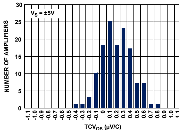
FIGURE 12. ISL28408 SOIC TCV_{OS} vs NUMBER OF AMPLIFIERS, V_S = \pm 5V
