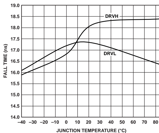
Figure 9. DRVH and DRVL Fall Times vs. Temperature
