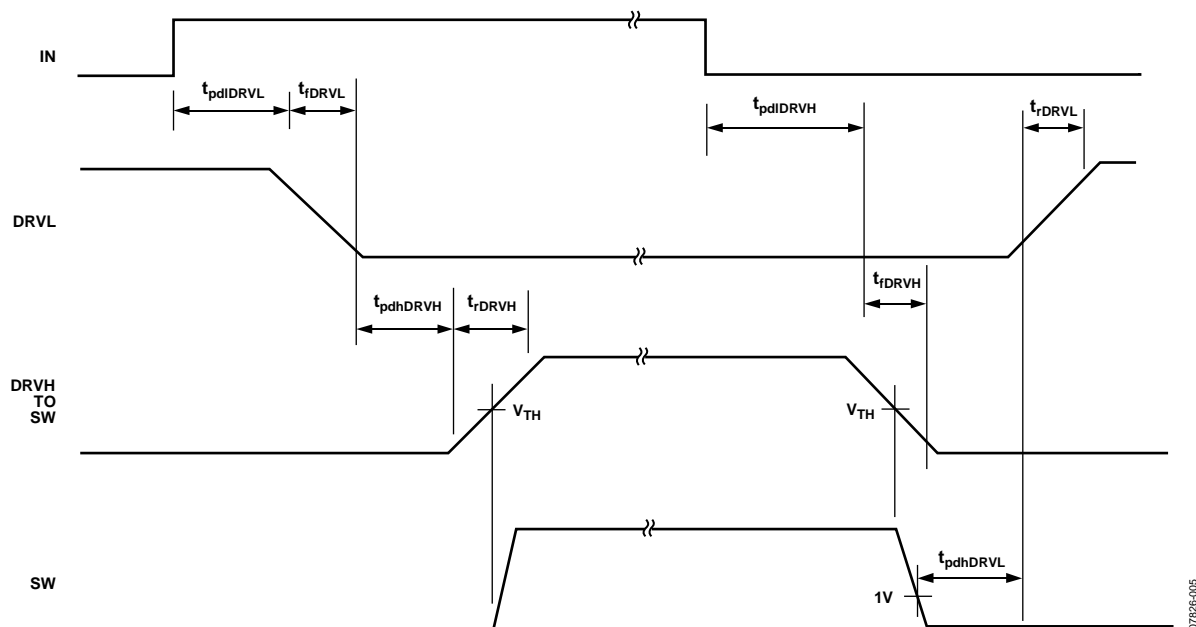
Figure 3. Timing Diagram
