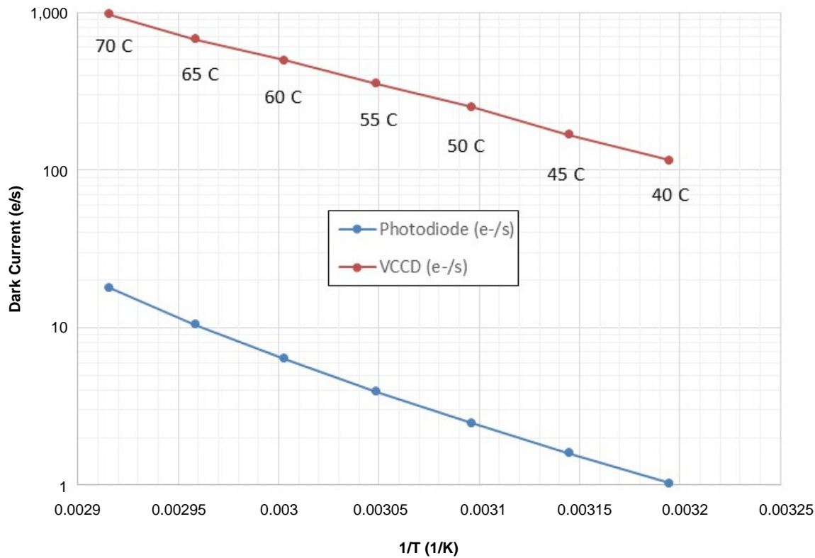
Figure 13. Dark Current vs. Temperature
