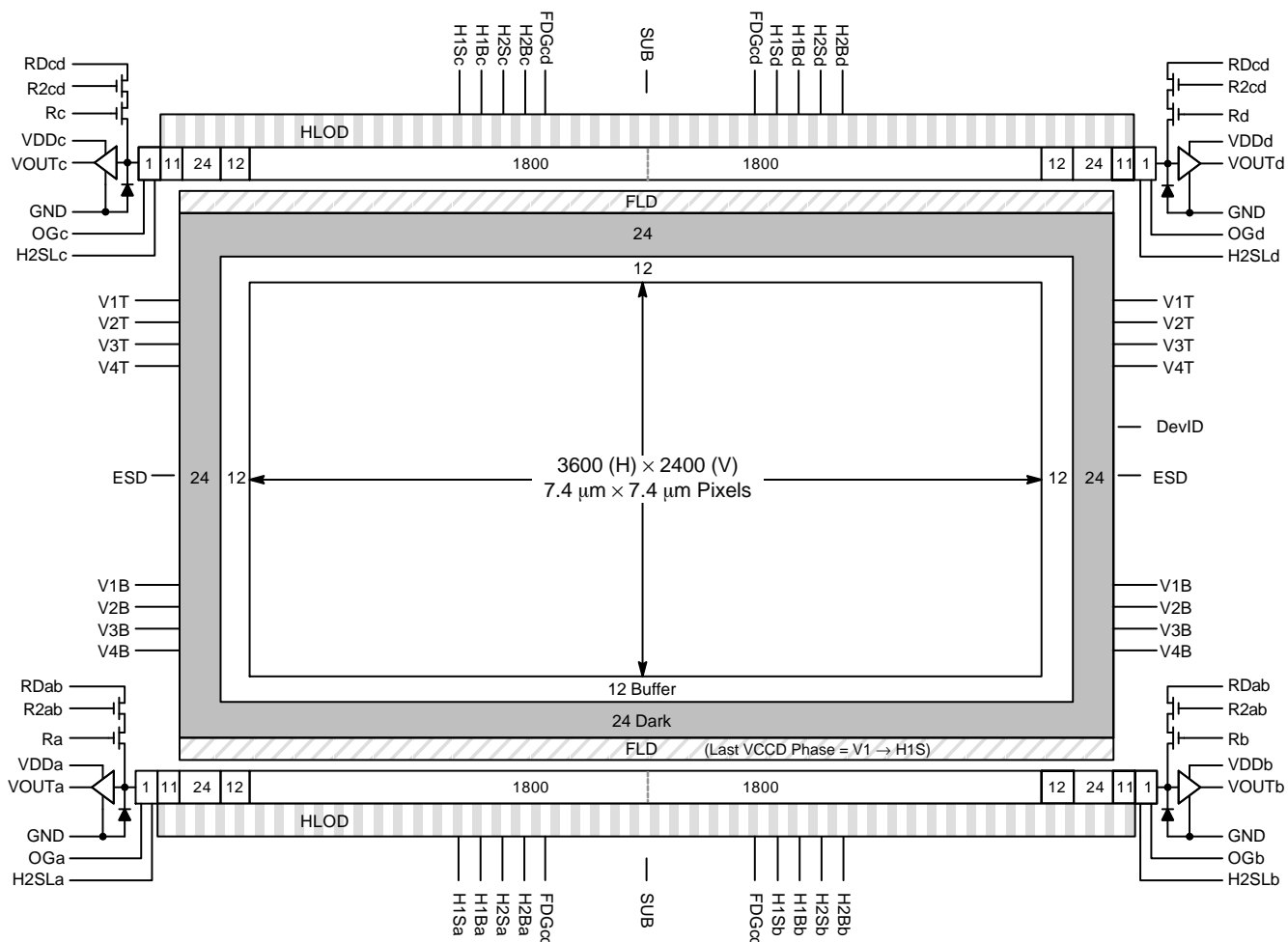
Figure 2. Block Diagram
