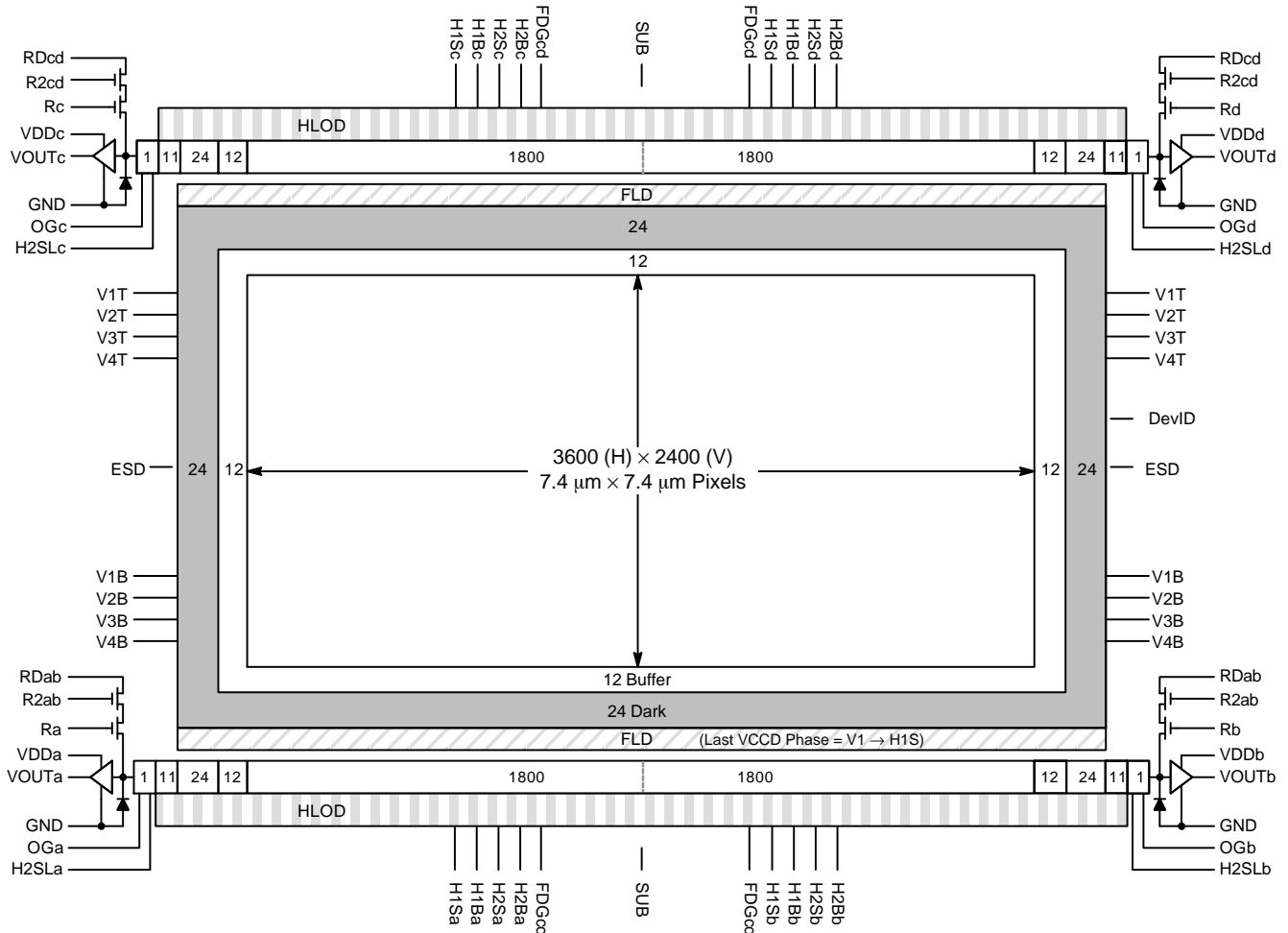
Figure 2. Block Diagram
