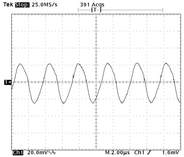
Fig-2.0V-5: Output voltage ripple (20mV/div.) for V_{out}=2.0V at full rated load current into a resistive load with external capacitance 47\mu F \times 4 ceramic + 1µF ceramic at V_{in}=5.0V .
