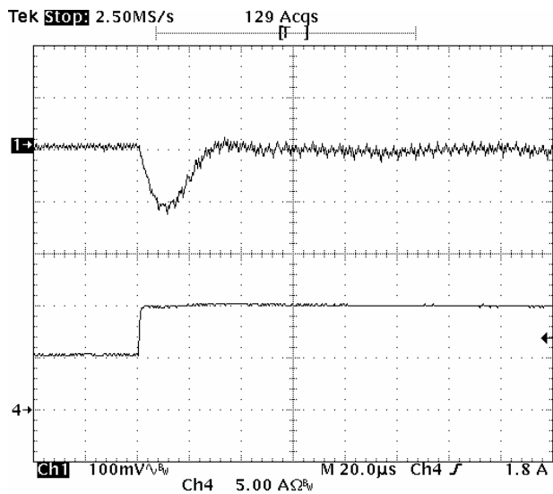
Fig-2.0V-6: Output voltage response for V_{out}=2.0V to positive load current step-change from 5A to 10A with slew rate of 5A/\mu s at V_{in}=5.0V . C_o=47\mu F \times 4 ceramic + 1µF ceramic.
