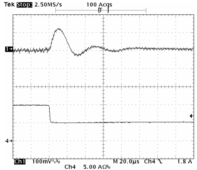
Fig-2.0V-7: Output voltage response for V_{out}=2.0V to positive load current step-change from 10A to 5A with slew rate of -5A/\mu s at V_{in}=5.0V . C_o=47\mu F \times 4 ceramic + 1µF ceramic.
