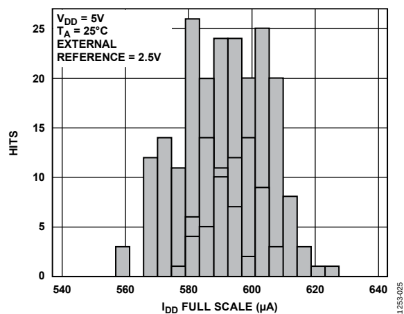
Figure 23. I_{DD} Histogram with External Reference
