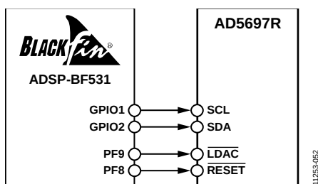
Figure 50. ADSP-BF531 Interface to the AD5697R
