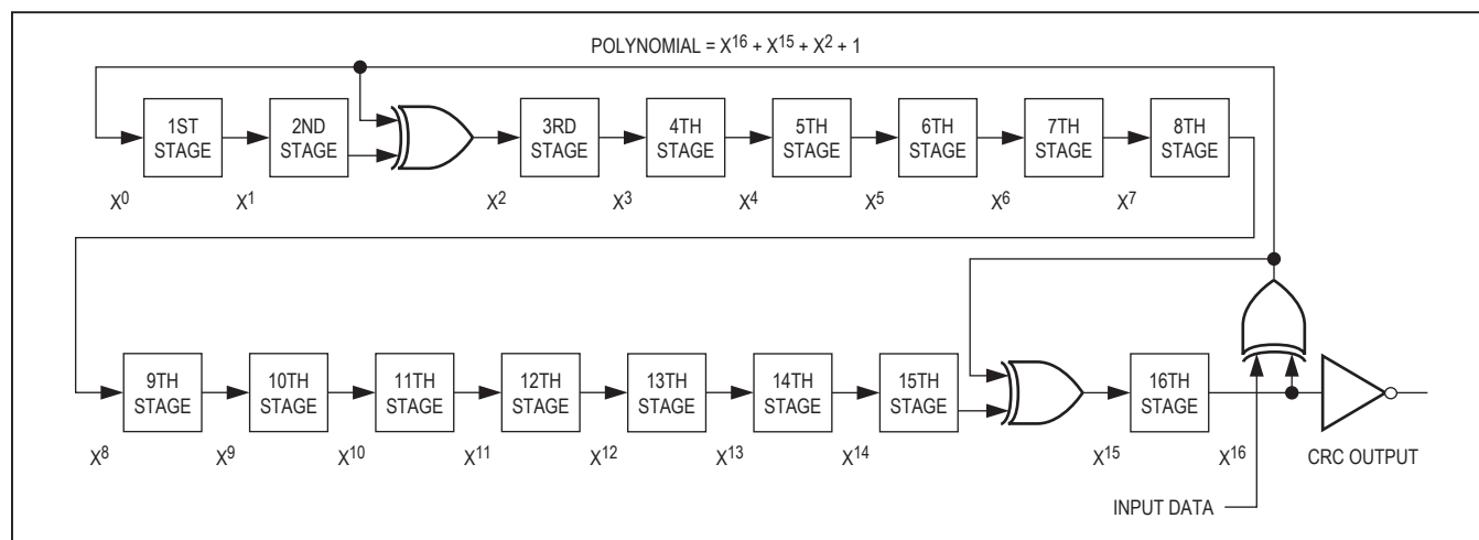
Figure 12. CRC-16 Generator
