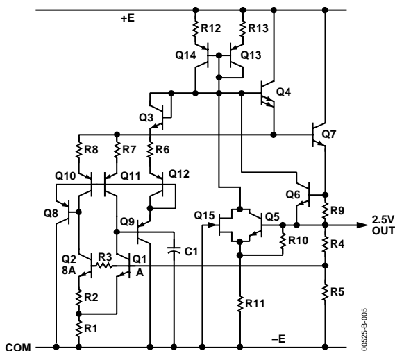
Figure 5. Schematic Diagram
