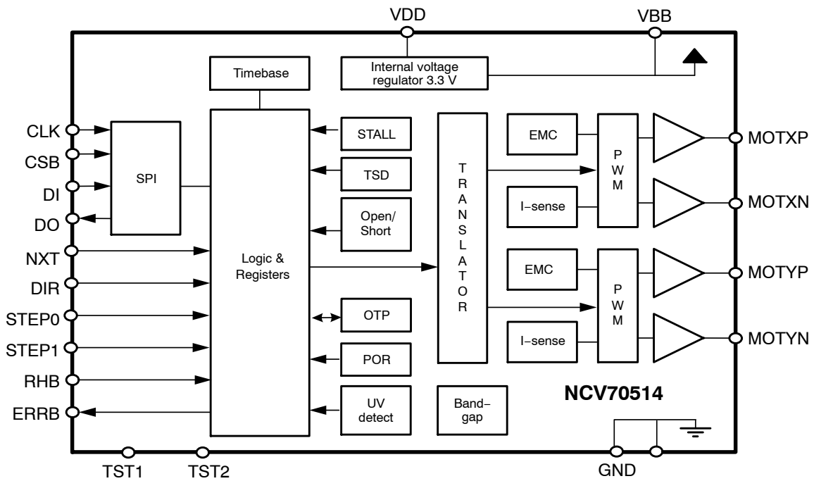
Figure 2. Block Diagram
