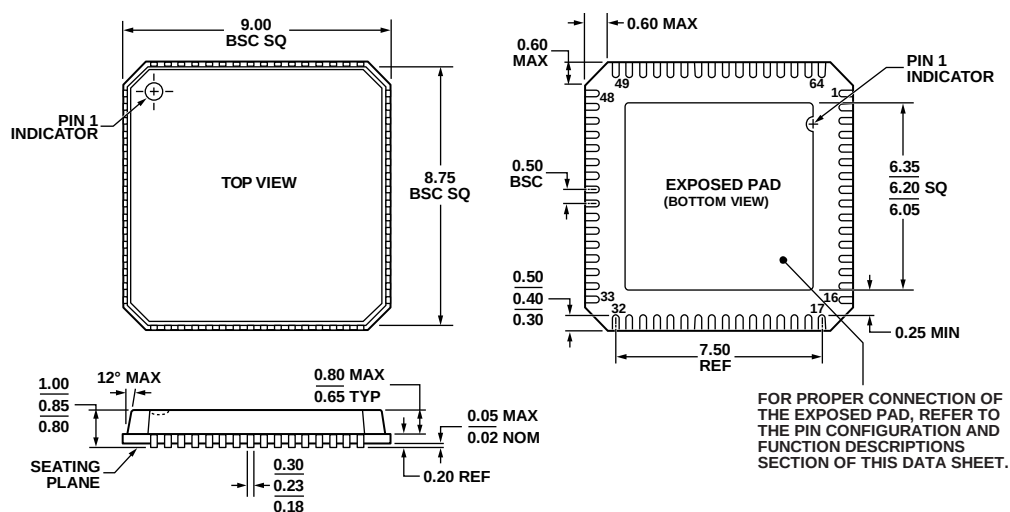
Figure 60. 64-Lead Lead Frame Chip Scale Package [LFCSP_VQ] 9 mm x 9 mm Body, Very Thin Quad (CP-64-4) Dimensions shown in millimeters
