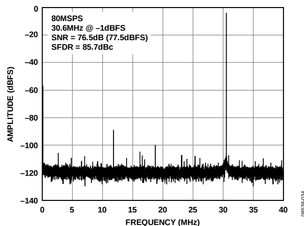
Figure 9. AD9269-80 Single-Tone FFT with f_{IN} = 30.6 MHz
