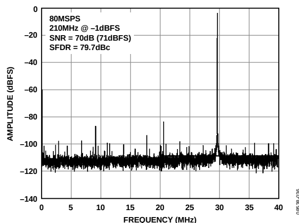
Figure 10. AD9269-80 Single-Tone FFT with f_{IN} = 210 MHz
