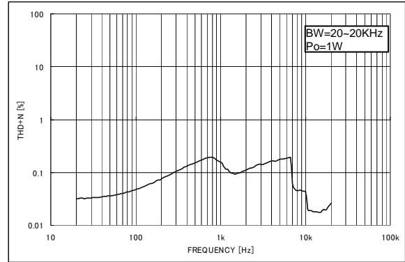
Fig.28 THD+N – Frequency
