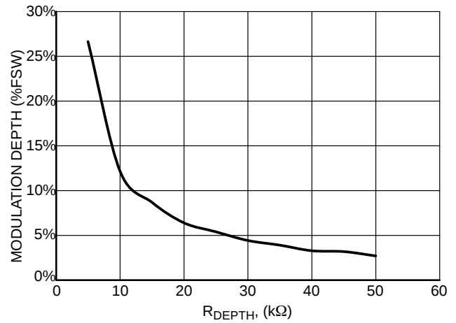
Figure 29. Modulation Depth vs. RDEPTH
