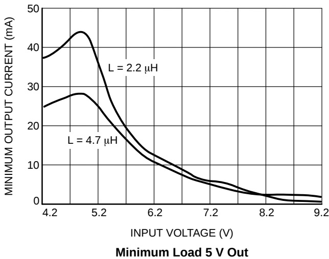
Minimum Load 5 V Out
