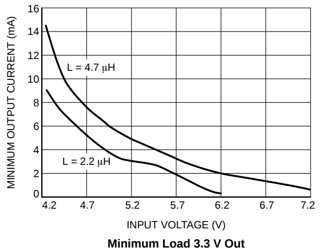
Minimum Load 3.3 V Out
