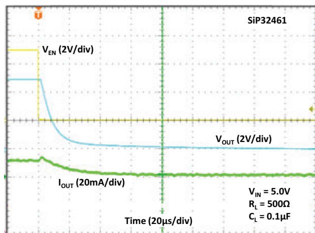
Fig. 40 - Turn-off Time
