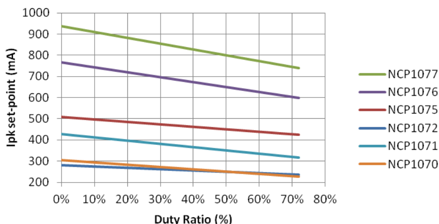
Figure 34. I_{PK} Set-point Varies with Power Switch On Time, Which is Caused by the Ramp Compensation
