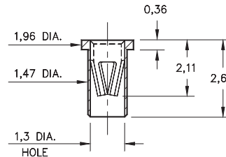
7305-0-15-XX-47-XX-10-0 Solder mount in 1,52 min. mounting hole Also available on 8mm wide carrier tape: 6,000 parts per 330mm reel. Order as: 7305-0-57-XX-47-XX-10-0
