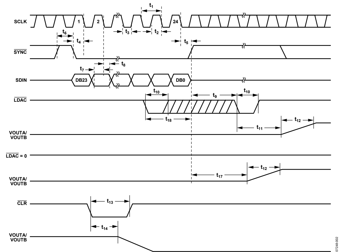
Figure 2. Serial Interface Timing Diagram
