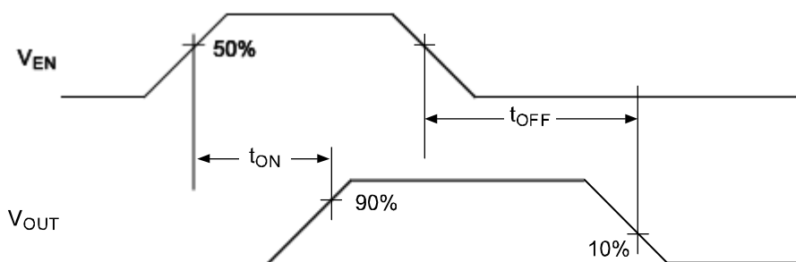
Figure 1a. MIC2546/47-1
