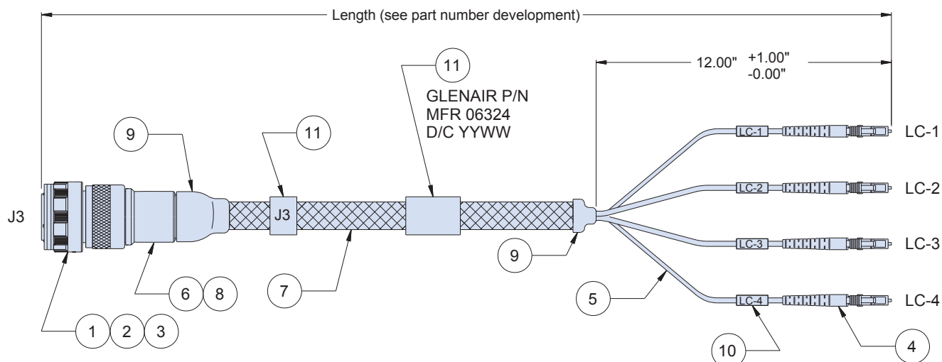
Connection Diagram
