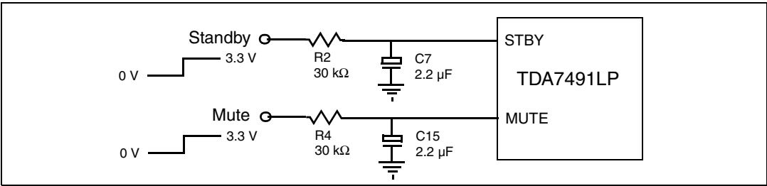
Figure 27. Standby and mute circuits
