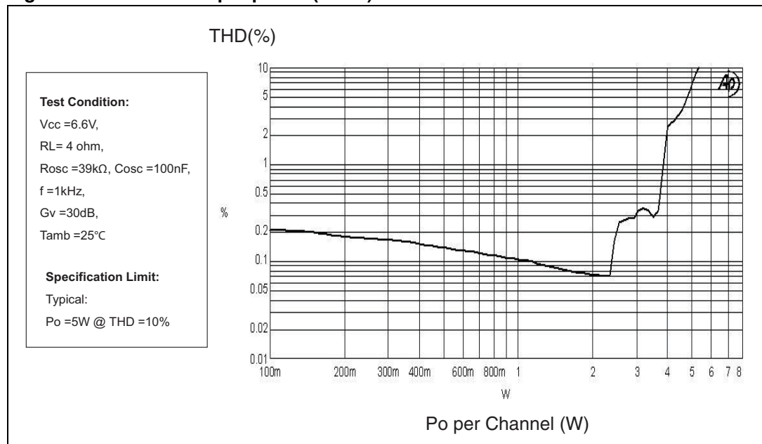
Figure 4. THD vs. output power (1 kHz)
