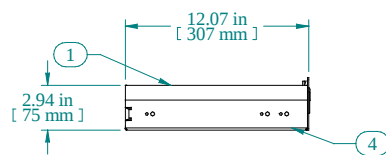
SIDE VIEW WITHOUT SHROUD
