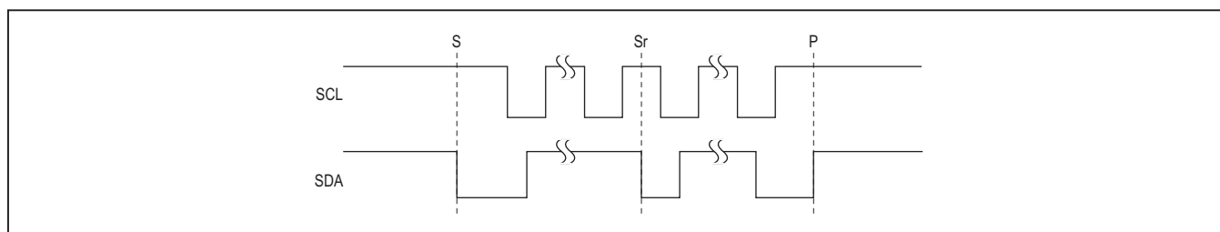
Figure 47. START, STOP, and REPEATED START Conditions
