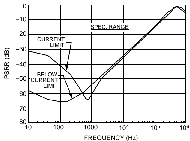
Figure 14. L8560 Typical Vcc Power Supply Rejection
