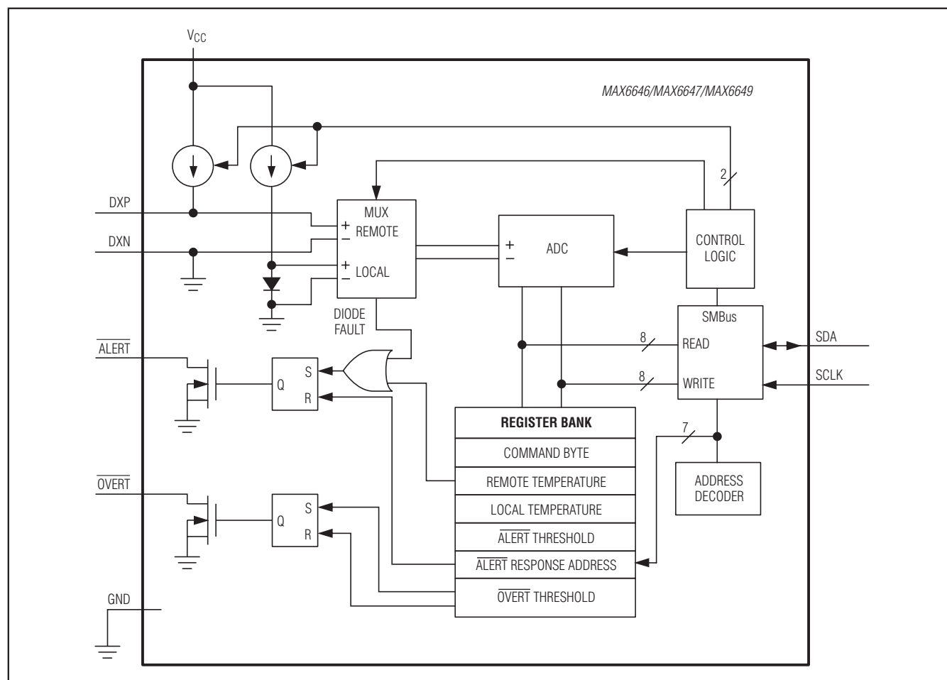
Functional Diagram
