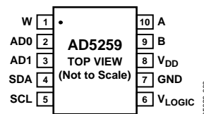
Figure 3. Pinout
