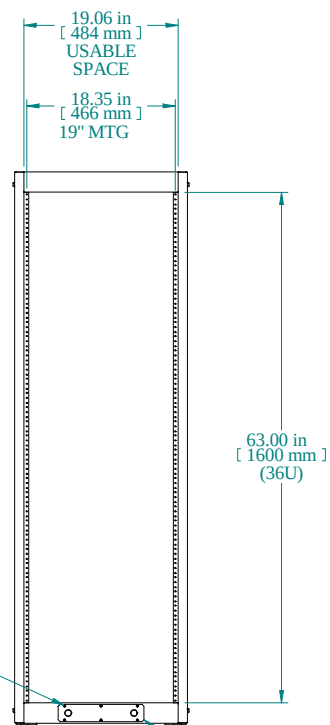
REAR VIEW
