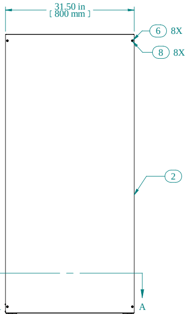
L.S. VIEW
