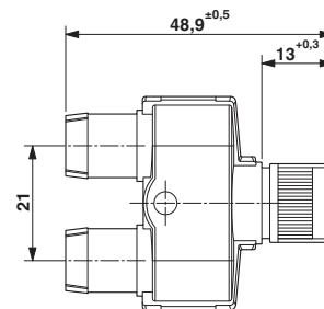
Dimensioned drawing
