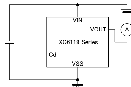
Circuit ⑥
