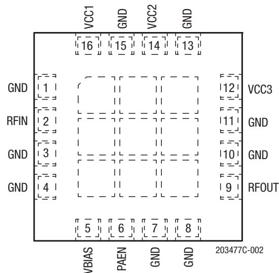
Figure 2. SKY66288-11 Pinout (Top View)
