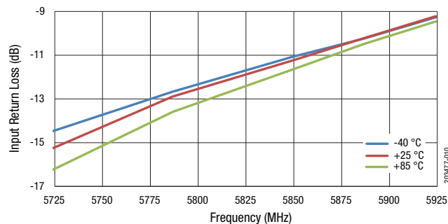
Figure 10. Input Return Loss @ High Band ( P_{IN} = -30 dB)
