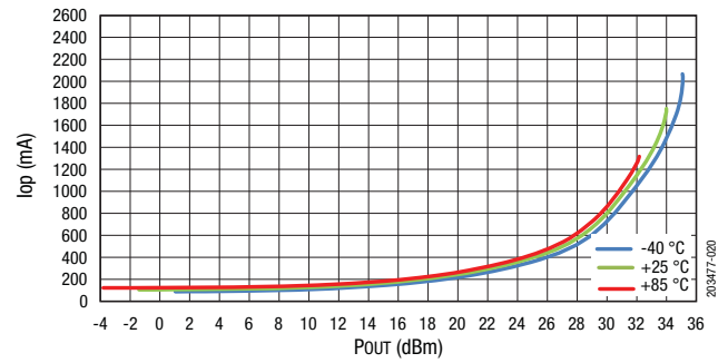
Figure 20. Total Current vs Output Power @ 5787.5 MHz
