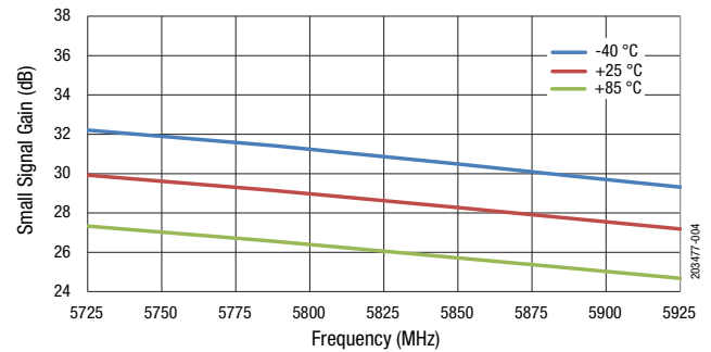
Figure 4. Small Signal Gain @ High Band (PIN = -30 dB)
