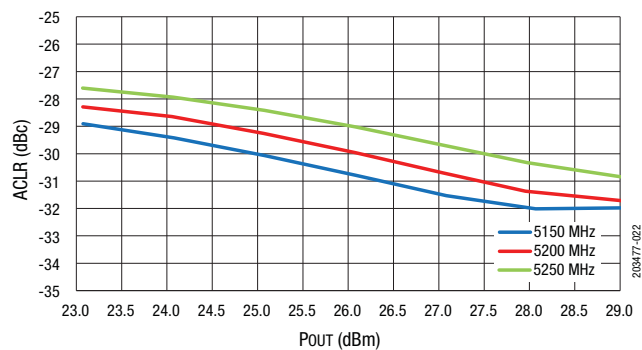
Figure 22. ACLR vs. Output Power for Low Band (LTE, 1x20 MHz, PAR = 8.5 dB)
