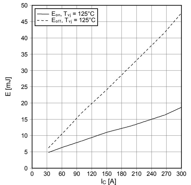
Schaltverluste IGBT-Wechselr. (typisch) switching losses IGBT-inverter (typical) E_{on} = f(I_c), E_{off} = f(I_c) V_{GE} = \pm 15\text{ V}, R_{Gon} = 8.2\ \Omega, R_{Goff} = 8.2\ \Omega, V_{CE} = 600\text{ V}
