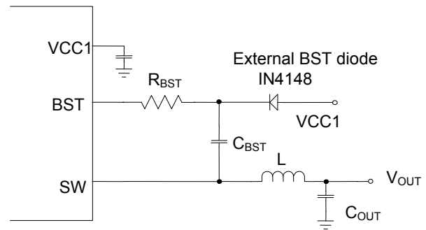
Figure 8: External Bootstrap Diode and Resistor
