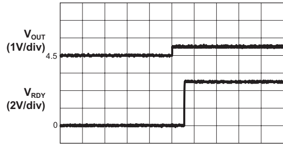
RDY Delay Time From Low to High ( V_{CC} = 5.0V , R_{SET} = 1.24M\Omega )
