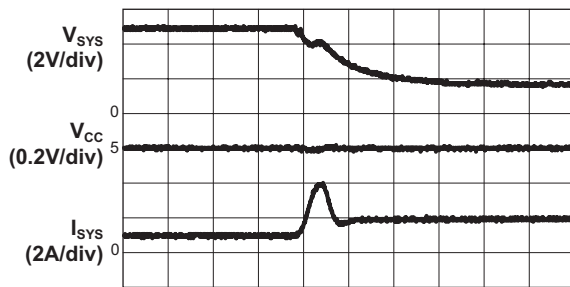
Current Limit Response ( V_{CC} = 5.0V , R_{SET} = 1.24M\Omega , R_{LOAD} = 5\Omega to 1\Omega )
