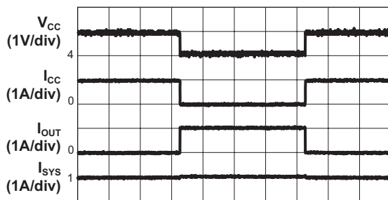
Discharge Path Switching ( V_{OUT} = 5.0V , R_{SET} = 1.24M\Omega , R_{ADJ} = 18.2k\Omega , V_{CC} = 5V to 4V , 1A Load)
