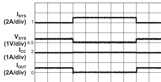
Load Transient ( V_{CC} = 5.0V , V_{OUT} = 2.0V , R_{SET} = 1.24M\Omega , I_{SYS} = 1A to 2A )
