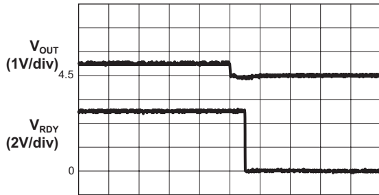
RDY Delay Time From High to Low ( V_{CC} = 5.0V , R_{SET} = 1.24M\Omega )
