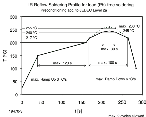
Fig. 9 - Vishay Lead (Pb)-free Reflow Soldering Profile (acc. to J-STD-020)
