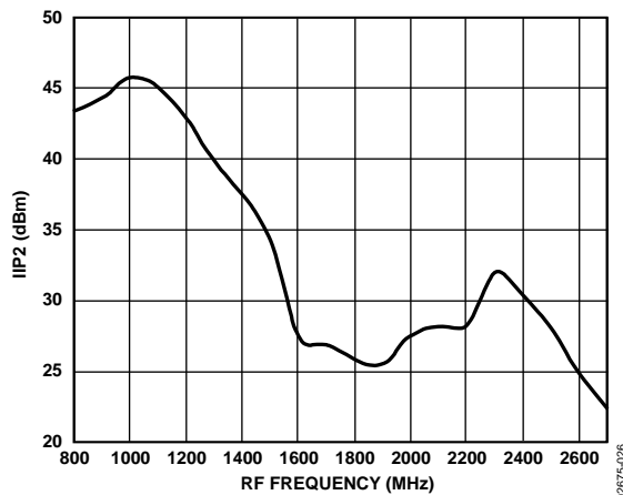
Figure 17. IIP2 vs. F_{LO} , V_{GIN} = 1.2 V, Baseband Tone1 = 5 MHz, -10 dBm, Baseband Tone2 = 6 MHz, -10 dBm, Temperature = 25°C, V_S = 5 V
