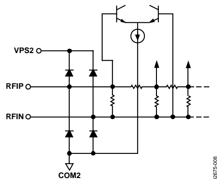
Figure 40. Circuit E
