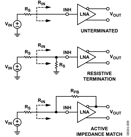
Figure 66. Input Resistance Matching
