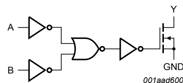
Figure 3. Logic diagram
