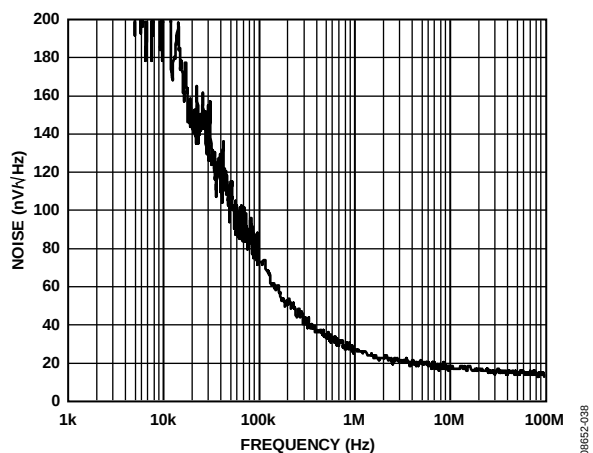
Figure 32. ADV3221 Output Noise vs. Frequency
