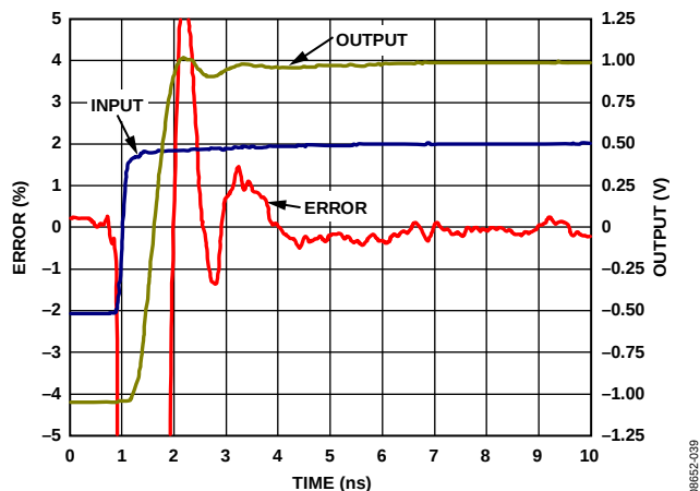
Figure 33. ADV3222 Settling Time, 2 V Step
