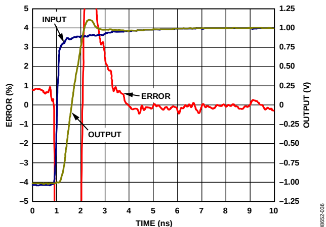
Figure 30. ADV3221 Settling Time, 2 V Step
