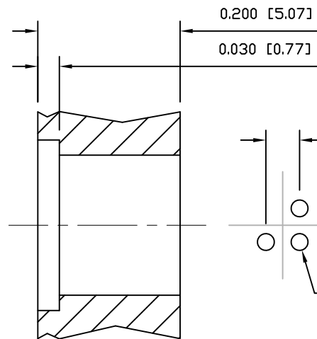
RECOMMENDED PANEL PCB
