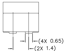
RECOMMENDED FOOTPRINT
