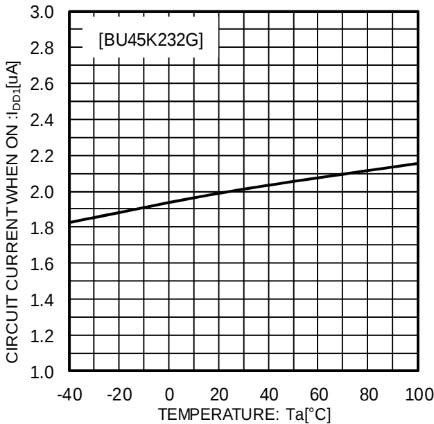
Fig.8 Circuit Current when ON ( V_{DD}=V_{DET}-0.2V ) V_{DD}=2.1V
