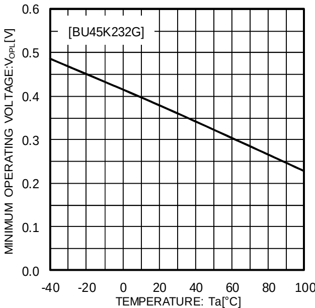
Fig.10 Operating Limit Voltage
