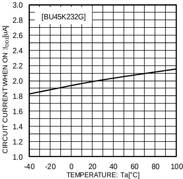
Fig.8 Circuit Current when ON ( V_{DD} = V_{DET} - 0.2V ) V_{DD} = 2.1V
