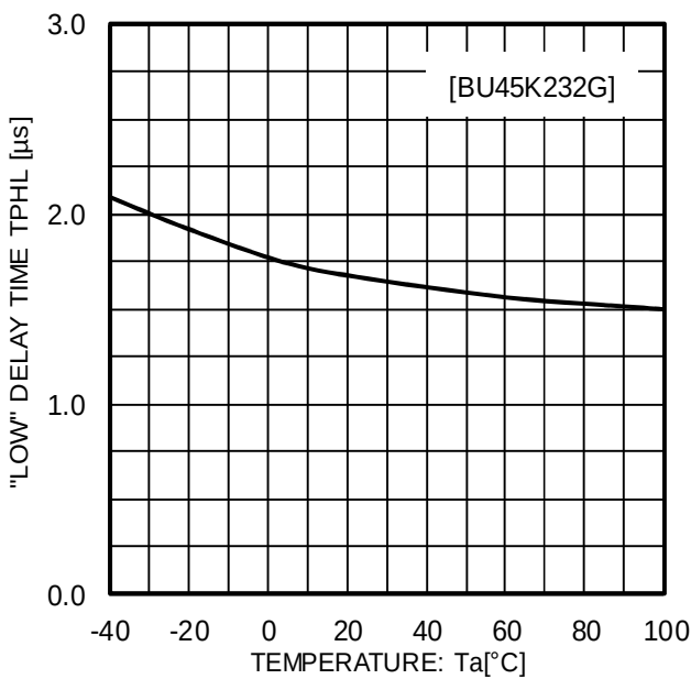
Fig.11 Output Delay Time "High" → "Low"
