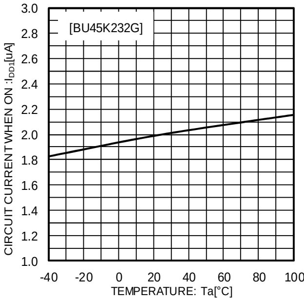
Fig.8 Circuit Current when ON ( V_{DD}=V_{DET}-0.2V ) V_{DD}=2.1V
