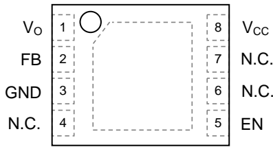
(VSON008X2030)
