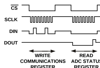
Figure 16. Serial Interface Signals—Registers Access
