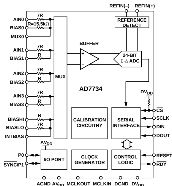
Figure 12. Block Diagram
