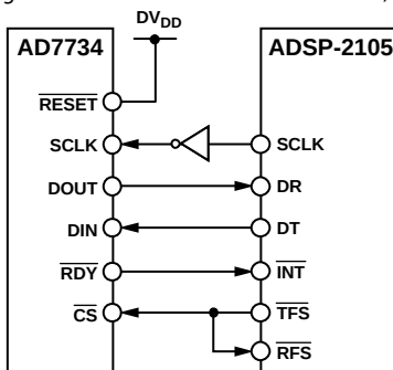
Figure 14. AD7734 to Host Device Interface, DSP
