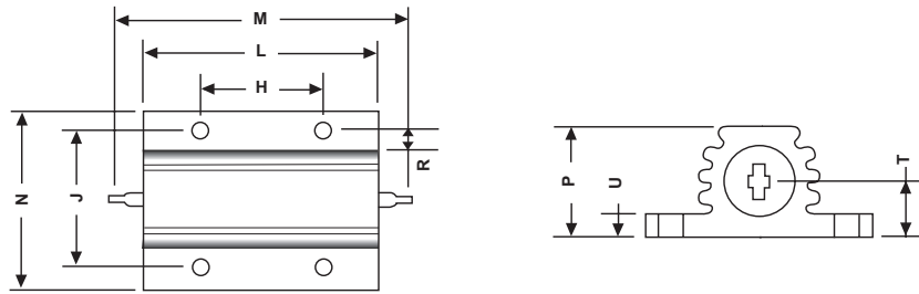
4 x Mounting Hole HSC75 - 4.4mm
