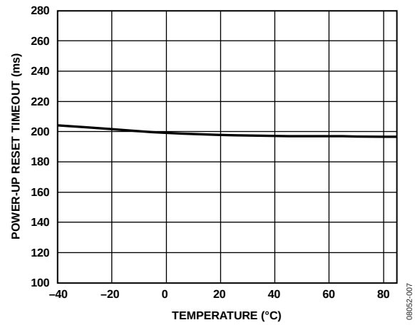
Figure 6. Power-Up Reset Timeout vs. Temperature
