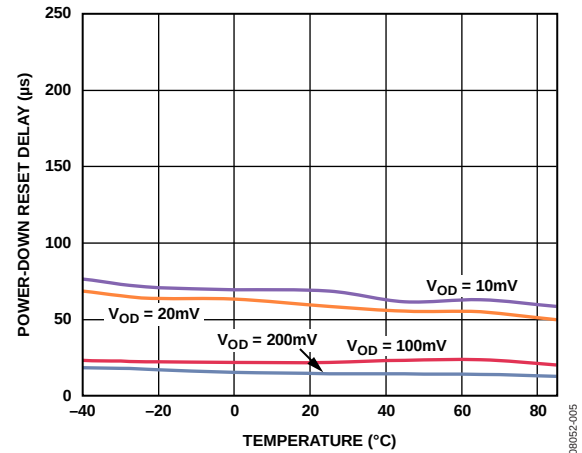
Figure 7. Power-Down Reset Delay vs. Temperature
