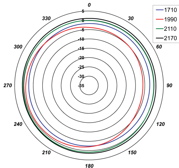
Horizontal Plane (1710-2170 MHz)
