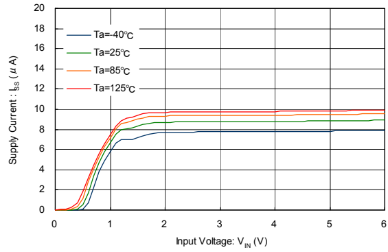
XC6130 ( V_{DF(T)}=3.0V )
